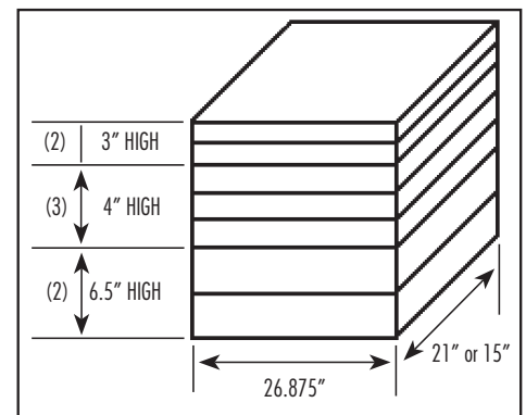
Drawer size diagram for 36" tall Tool Cabinet
